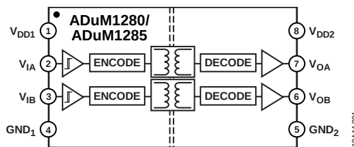
Figure 1. ADuM1280/ADuM1285
