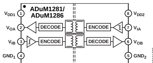
Figure 2. ADuM1281/ADuM1286
